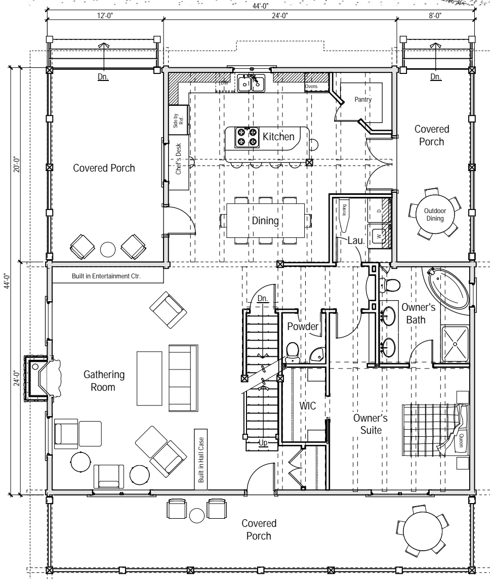
Main Level Plan
